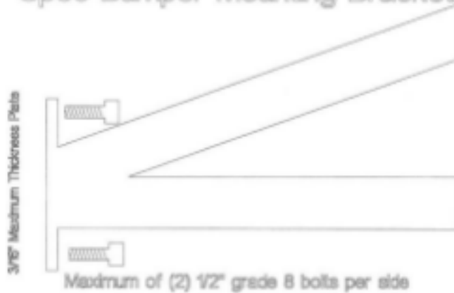
Spec Bumper Mounting Bracket
